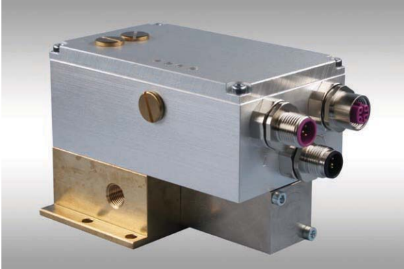
减压阀
